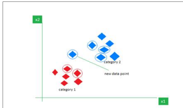
Figure 4. KNN Classifier [37].
